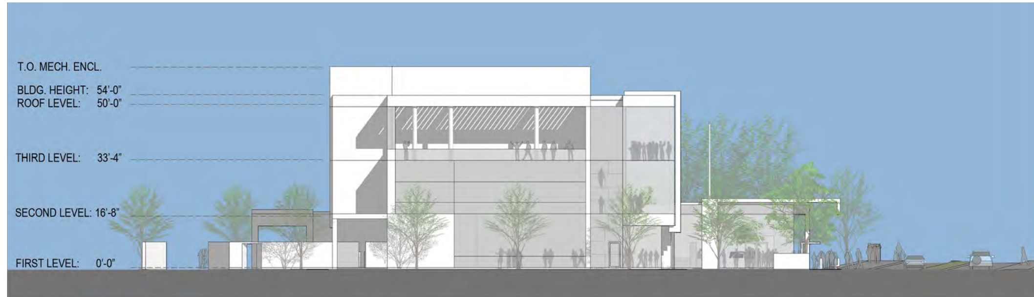
South Elevation
