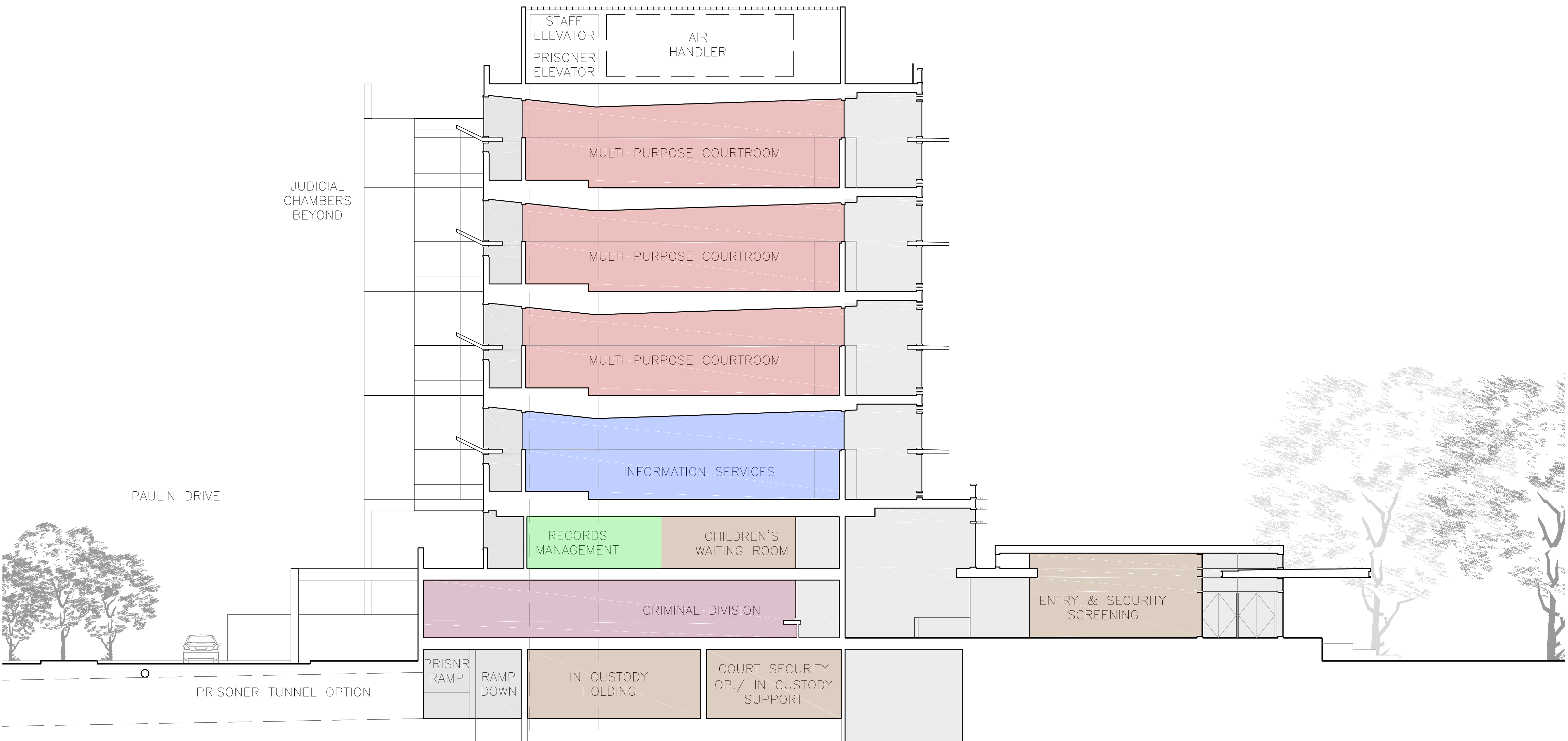
Building Section
