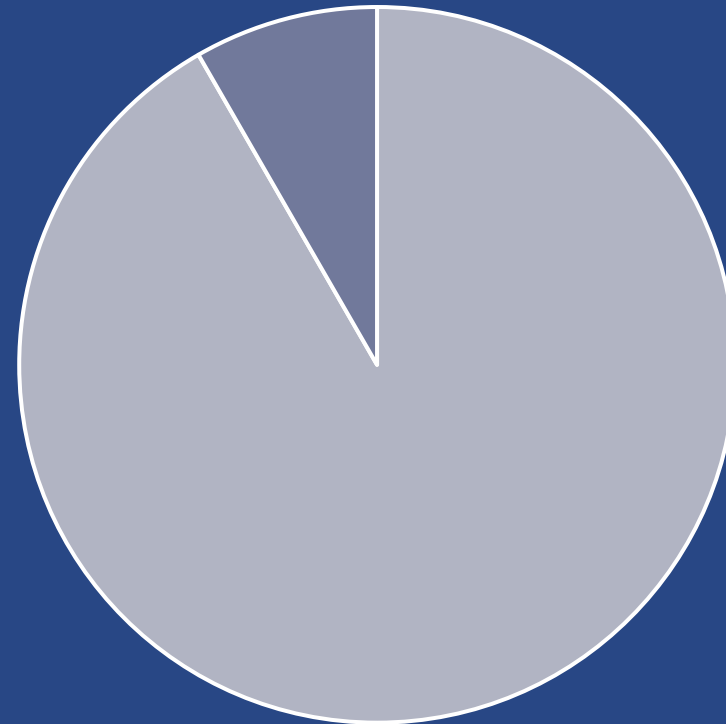
Distributed Collections
