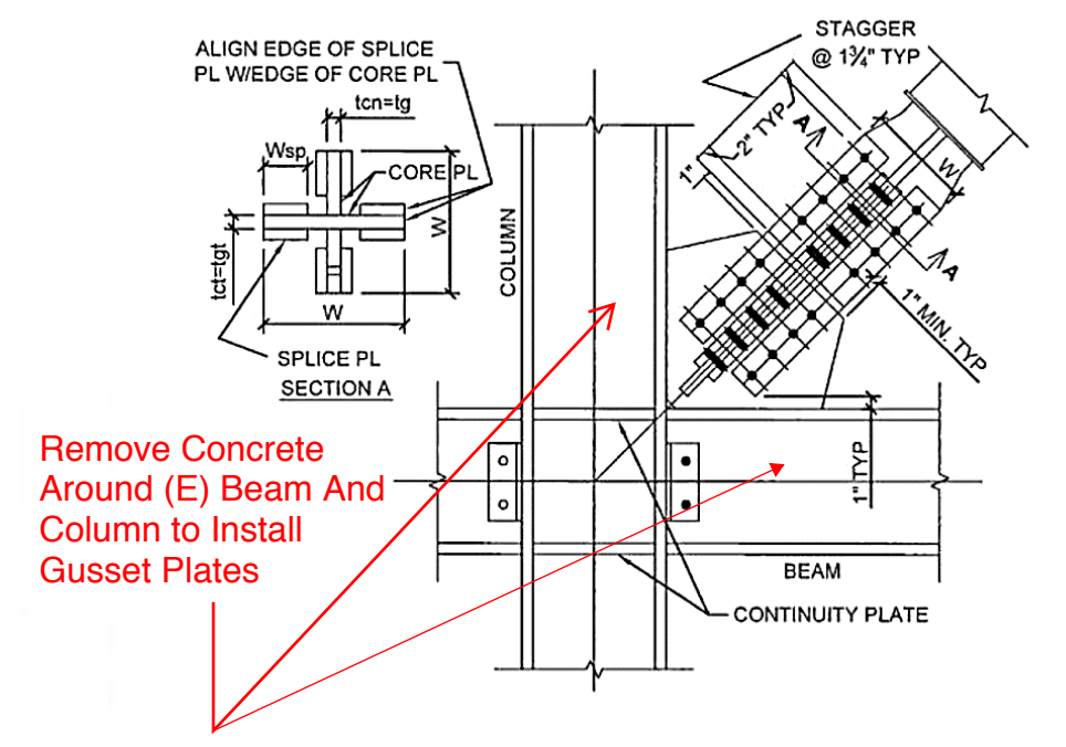
BRBF CONNECTION DETAIL DETAIL BY COREBRACE
