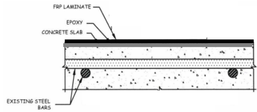
DETAIL 4: Bi-directional FRP Laminates on Slab for Diaphragm Retrofit
