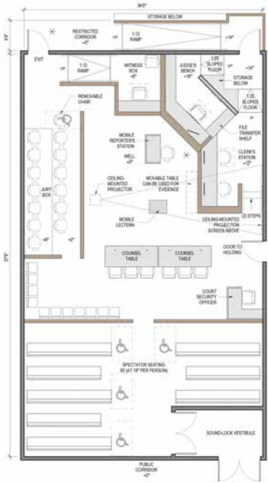
Figure 22.6 Typical Large Trial Courtroom—Corner Bench A
