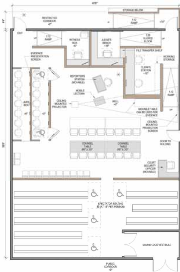
Figure 22.10 Typical Large Trial Courtroom—Center Bench D
