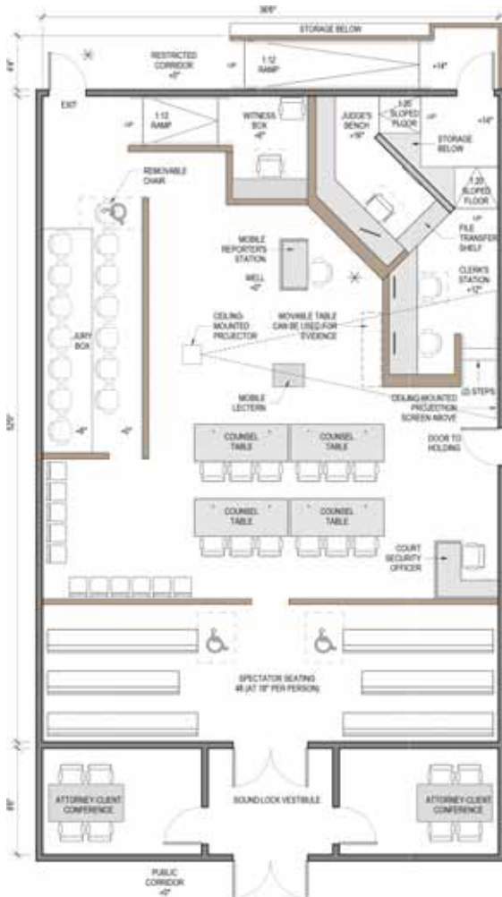
Figure 22.7 Typical Trial Courtroom—Corner Bench B
