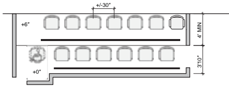
Figure 5.9 Jury Box Plan
