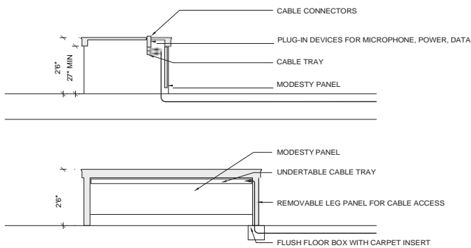
Figure 5.12 Counsel Table Section
