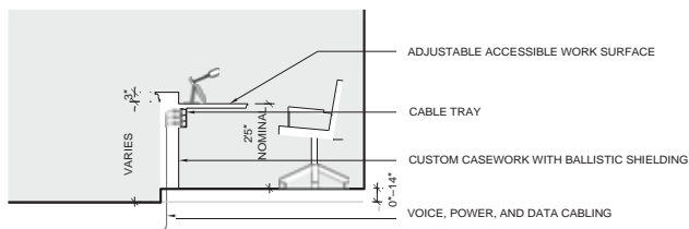
Figure 5.6 Clerk Station Section
