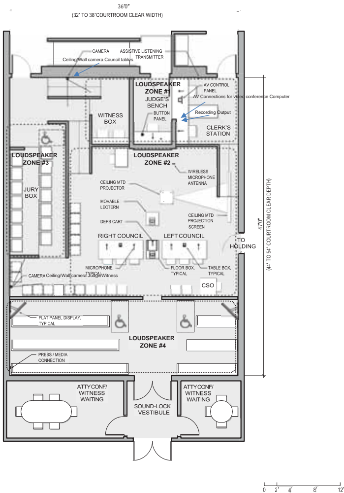
Figure 18.2 Typical Courtroom, Center Bench—A/V Requirement
