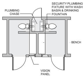
Figure 8.4 Single Holding Cells
