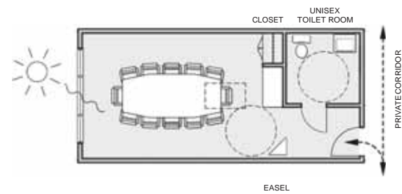
Figure 5.19 Jury Deliberation Room 300 SF JUDICIAL COUNCIL OF CALIFORNIA • CALIFORNIA TRIAL COURT FACILITIES STANDARDS • 2020
