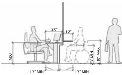
Figure 6.5 Universal Height Counter
