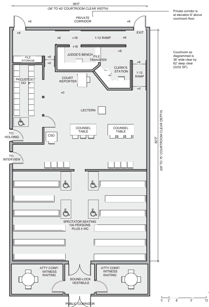
Figure 5.23 Arraignment Courtroom (Central Bench)
