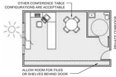
Figure 5.15 Judge's Chamber Plan
