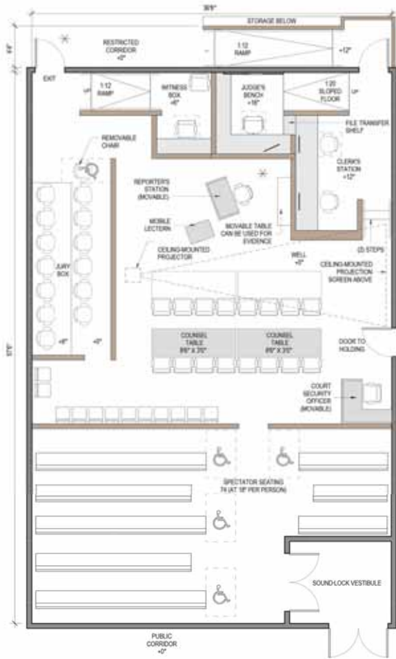
Figure 22.4 Typical Large Trial Courtroom—Center Bench B
