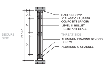
2 ATTORNEY AND IN-CUSTODY WINDOW SECTION
