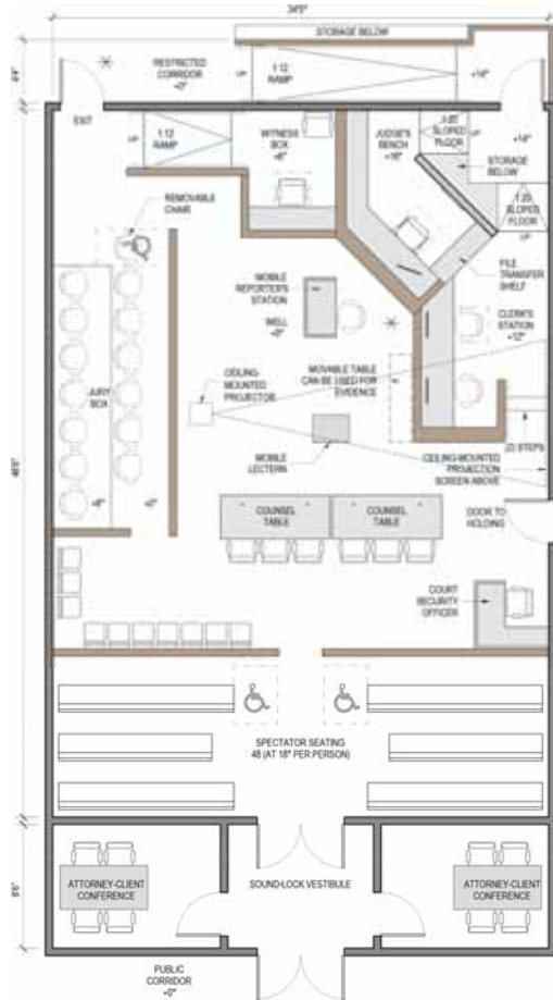
Figure 22.5 Typical Trial Courtroom—Corner Bench A
