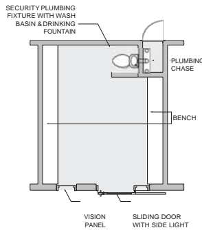
Figure 8.5 Group Holding Cell
