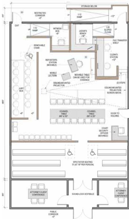
Figure 22.3 Typical Trial Courtroom—Center Bench B
