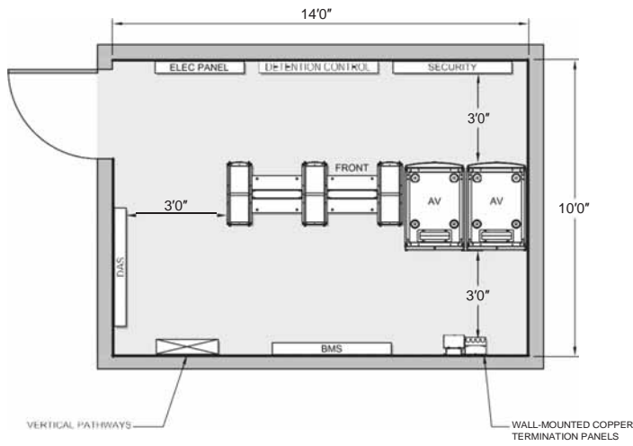
Figure 17.3 IDF Serving Two Courtrooms
