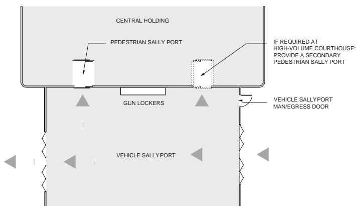
Figure 8.1 Vehicle Sally Port
