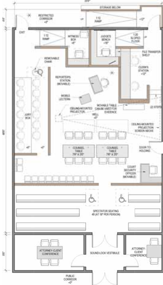
Figure 22.1 Typical Trial Courtroom—Center Bench A
