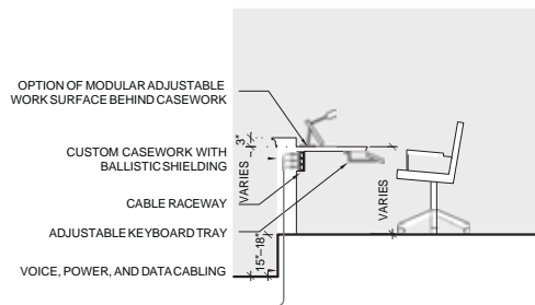
Figure 5.3 Judge's Bench Section
