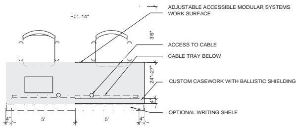
Figure 5.5 Clerk Station Plan
