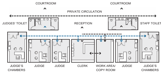
Figure 5.16 Clustered Chamber Layout
