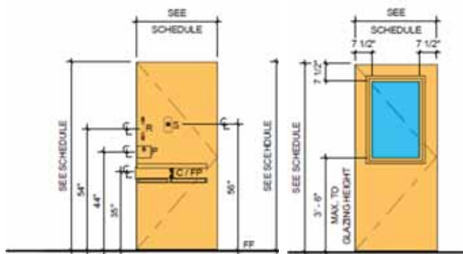
Figure 8.9 Center Line Height of Cuff Pass Figure 8.409 Glazed Opening and Center Line Height of Cuff Pass in Detention Door
