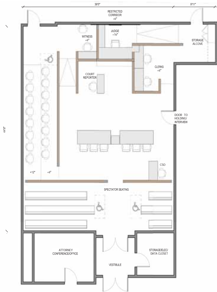
Figure 22.11 San Diego Central Courthouse, Trial Courtroom—Center Bench
