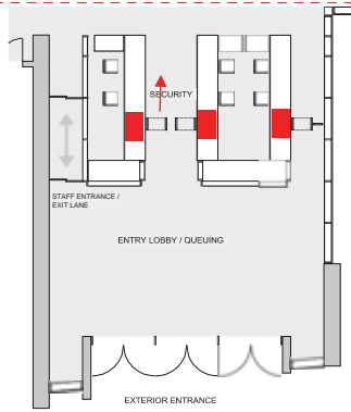
Figure 9.3 Screening Station Diagram
