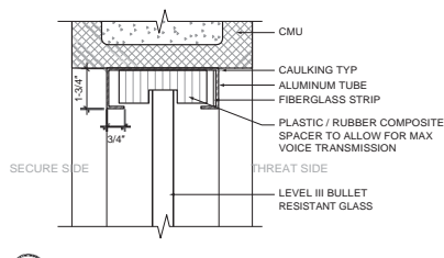
5 ATTORNEY AND IN-CUSTODY WINDOW TOP DETAIL
