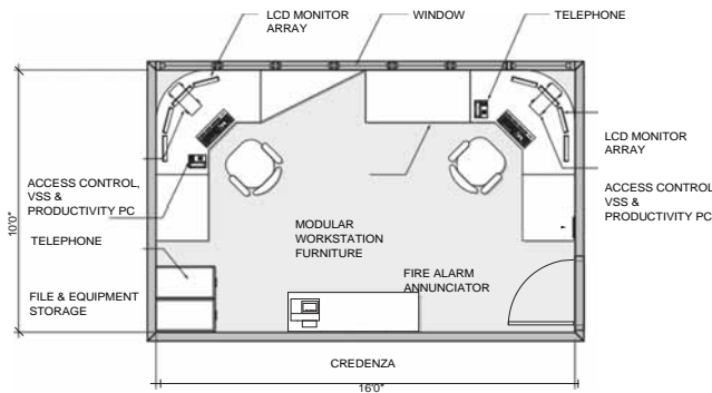
Figure 4.4 Plan of Security Operations Center
