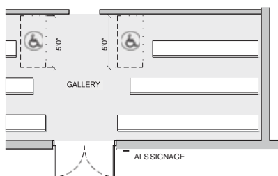
Figure 5.13 Bench-Type Spectator Seating
