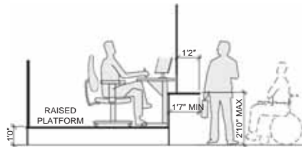
Figure 6.4 Transaction Height Counter
