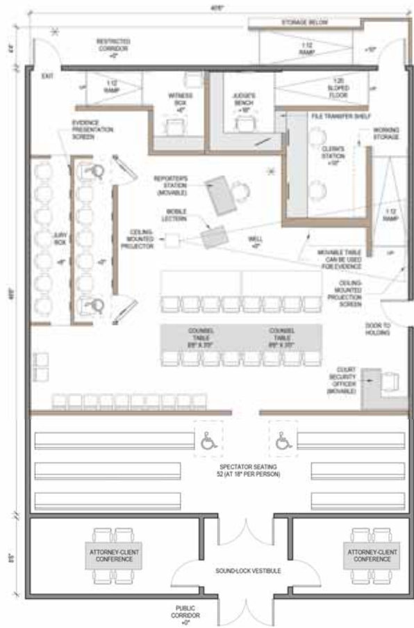
Figure 22.9 Typical Large Trial Courtroom—Center Bench C
