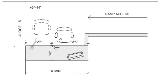
Figure 5.7 Witness Box Plan
