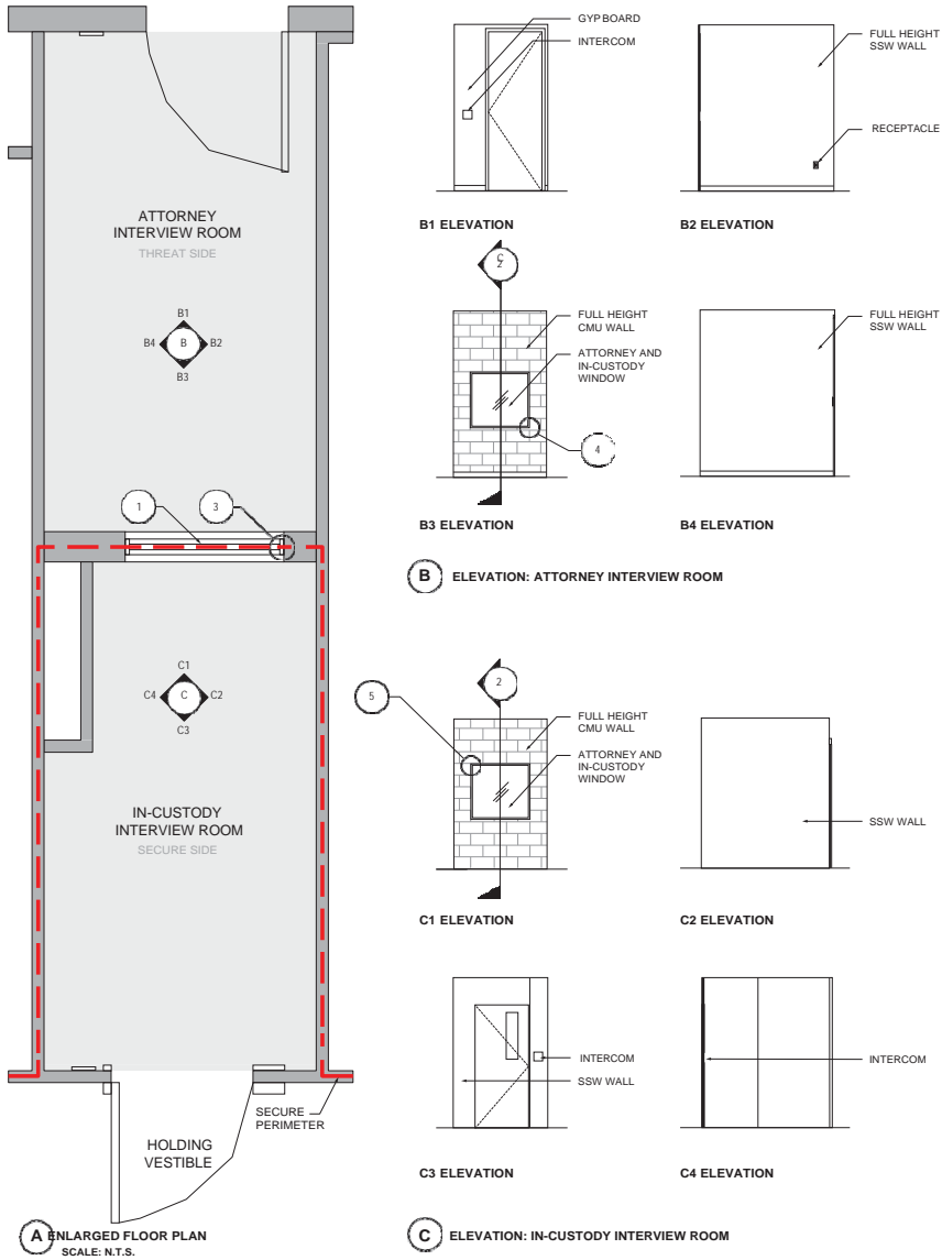
Figure 25.2 As-Built Drawing (not to scale)
