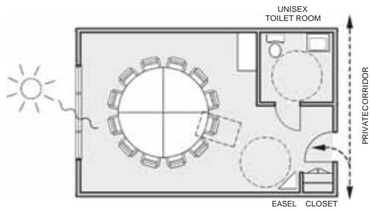
Figure 5.17 Jury Deliberation Room 400 SF
