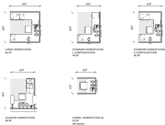
Figure 2.4 Open Plan Workstations*
