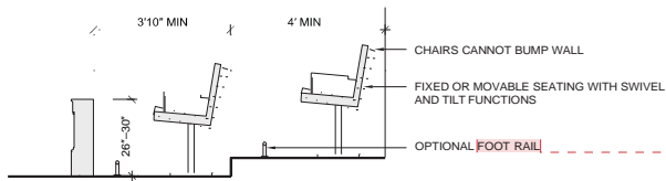
Figure 5.10 Jury Box Section
