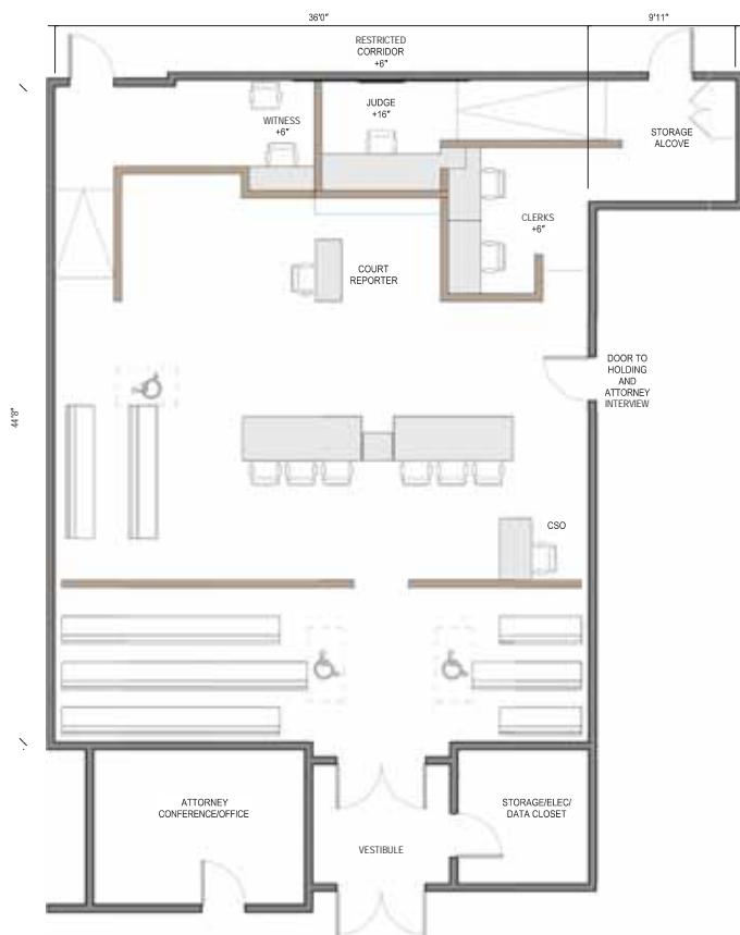
Figure 22.17 San Diego Central Courthouse, Family Courtroom—Center Bench
