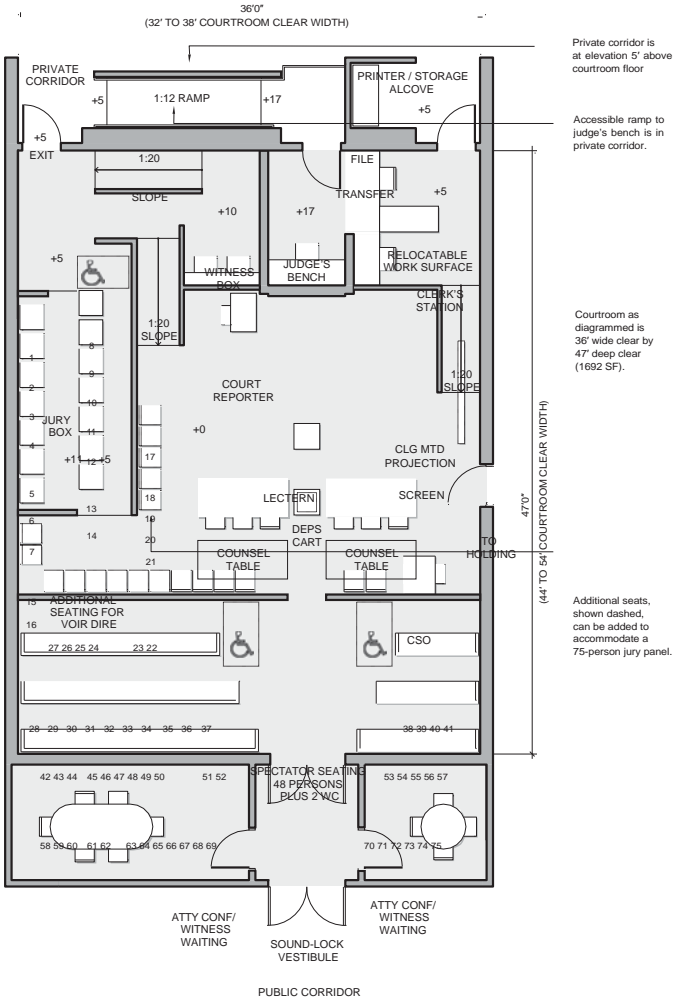
Figure 5.21 Multipurpose Courtroom (Central Bench—Asymmetrical)
