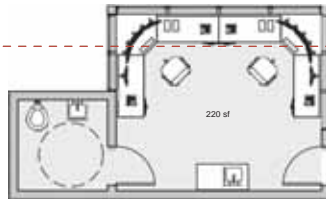
Figure 8.2 Detention Control Room
