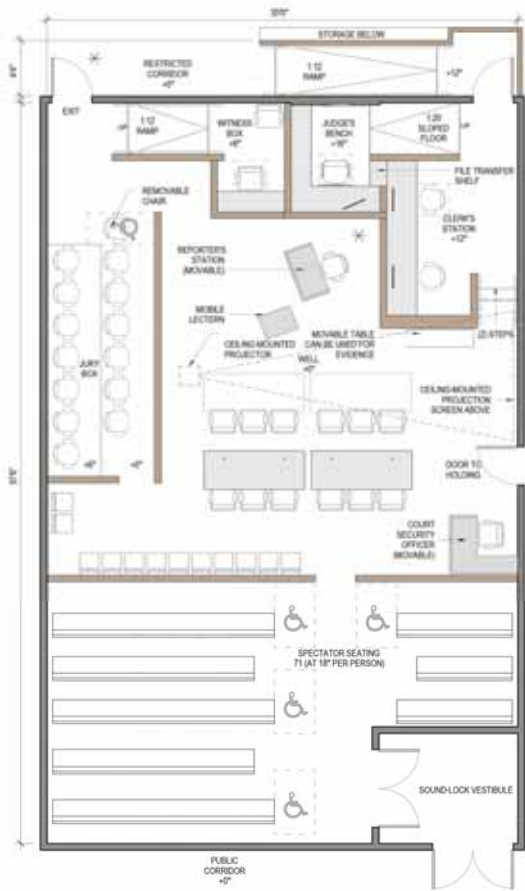
Figure 22.2 Typical Large Trial Courtroom—Center Bench A
