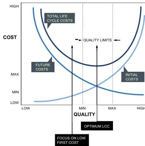
Figure 21.1 Life Cycle Cost Curve
