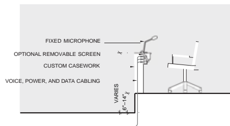
Figure 5.8 Witness Box Section
