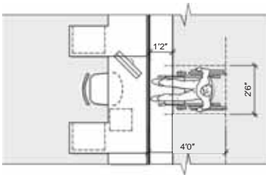
Figure 6.4 Transaction Height Counter
