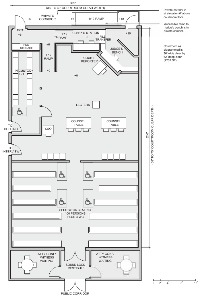
Figure 5.22 Arraignment Courtroom (Corner Bench)
