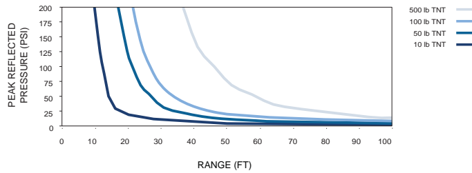
Figure 4.2 Peak Pressure Decay with Distance
