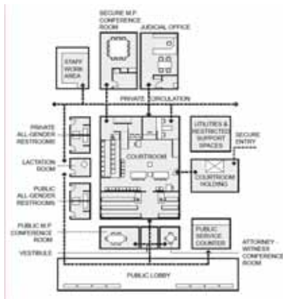
Figure 2.7 Illustration of One-Courtroom Courthouse Organization JUDICIAL COUNCIL OF CALIFORNIA • CALIFORNIA TRIAL COURT FACILITIES STANDARDS • 2020
