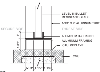
4 ATTORNEY AND IN-CUSTODY WINDOW BASE DETAIL
