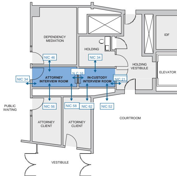
Figure 25.1 Airborne Sound Isolation Measurement
