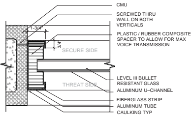
3 ATTORNEY AND IN-CUSTODY WINDOW SIDE DETAIL
