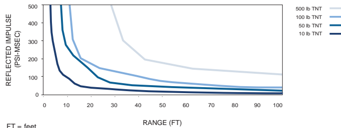
Figure 4.3 Impulse Decay with Distance
