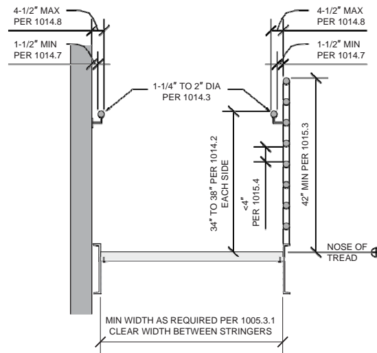
Figure 11.1 Egress Width Measurement Method
