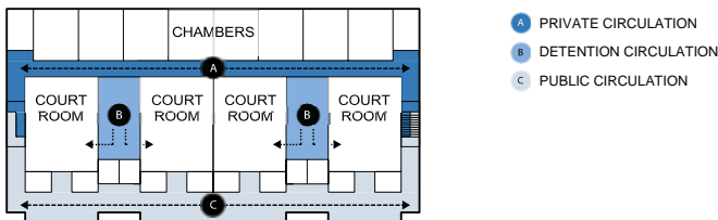
Figure 2.2 Three Circulation Zones
