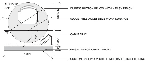
Figure 5.2 Judge's Bench Plan
