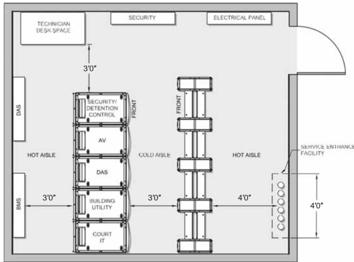
Figure 17.2 Typical Smaller Courthouse MDF Layout
