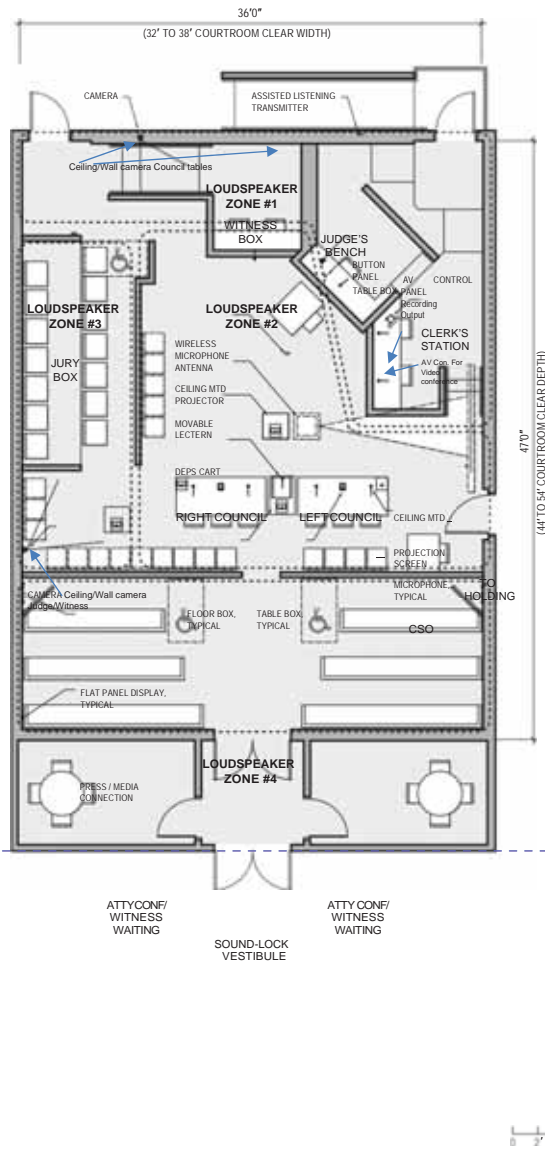
Figure 18.1 Typical Courtroom, Corner Bench—A/V Requirement
