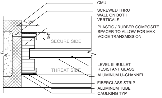
3 ATTORNEY AND IN-CUSTODY WINDOW SIDE DETAIL
