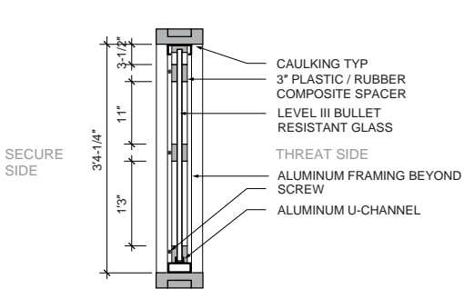
2 ATTORNEY AND IN-CUSTODY WINDOW SECTION
