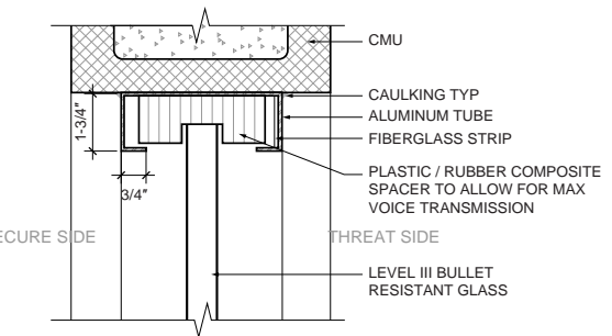
5 ATTORNEY AND IN-CUSTODY WINDOW TOP DETAIL
