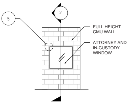
C1 ELEVATION
