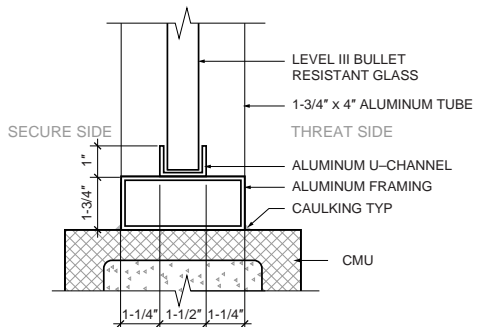
4 ATTORNEY AND IN-CUSTODY WINDOW BASE DETAIL
